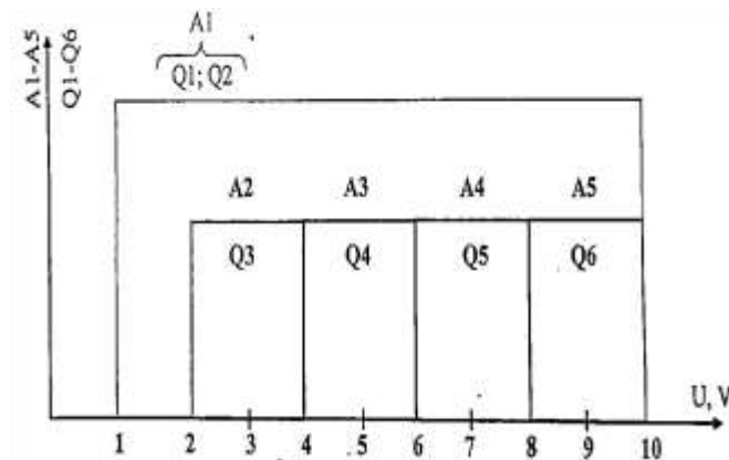
Fig.2 Working digits of A1-A5 resistance element and output signals (Q1-Q6)
