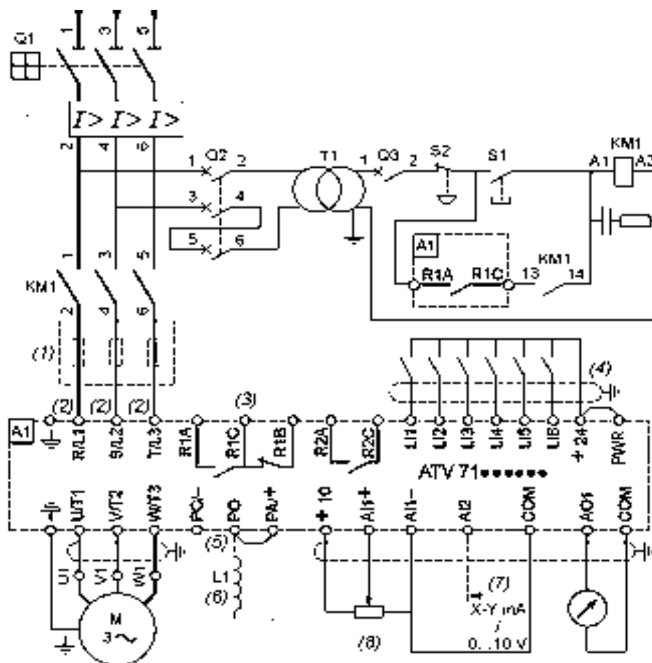
Fig.1 Connection and control scheme of the Altivar 71 type frequency converter to the asynchronous motor
